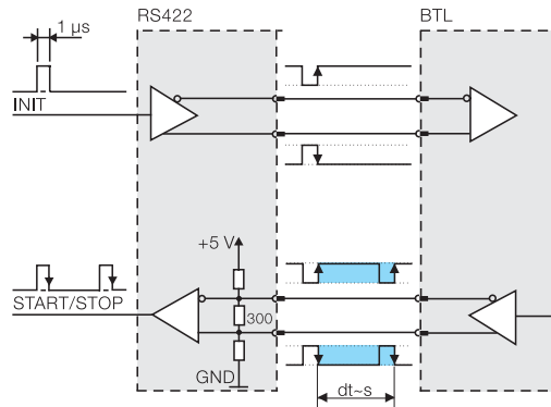
Block diagram of the P-interface
