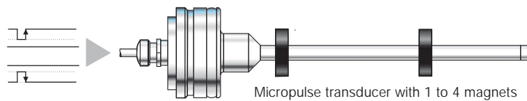
Micropulse transducer with 1 to 4 magnets
