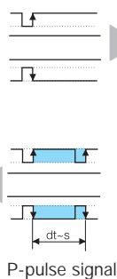
P-pulse signal
